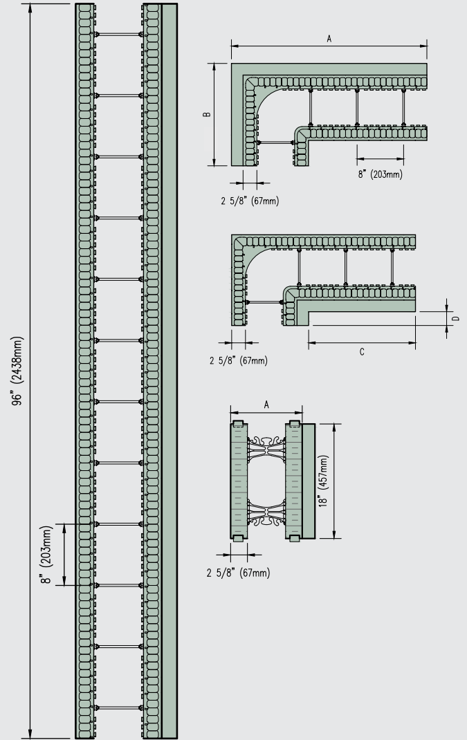
Information in the charts and the images show the 6" (152mm) form only
