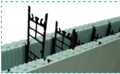
Close view of insert webs - available in 4"-12" (102-305mm) sizes
