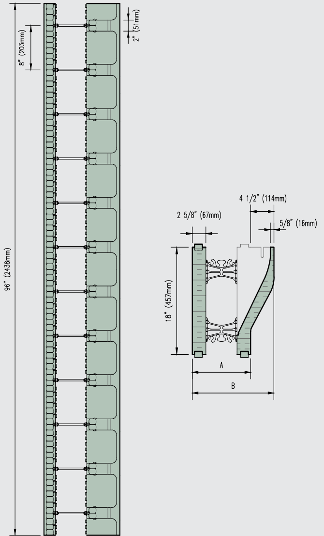
Assembled 96" (2438mm) Molded Brick Ledge Shown Above
