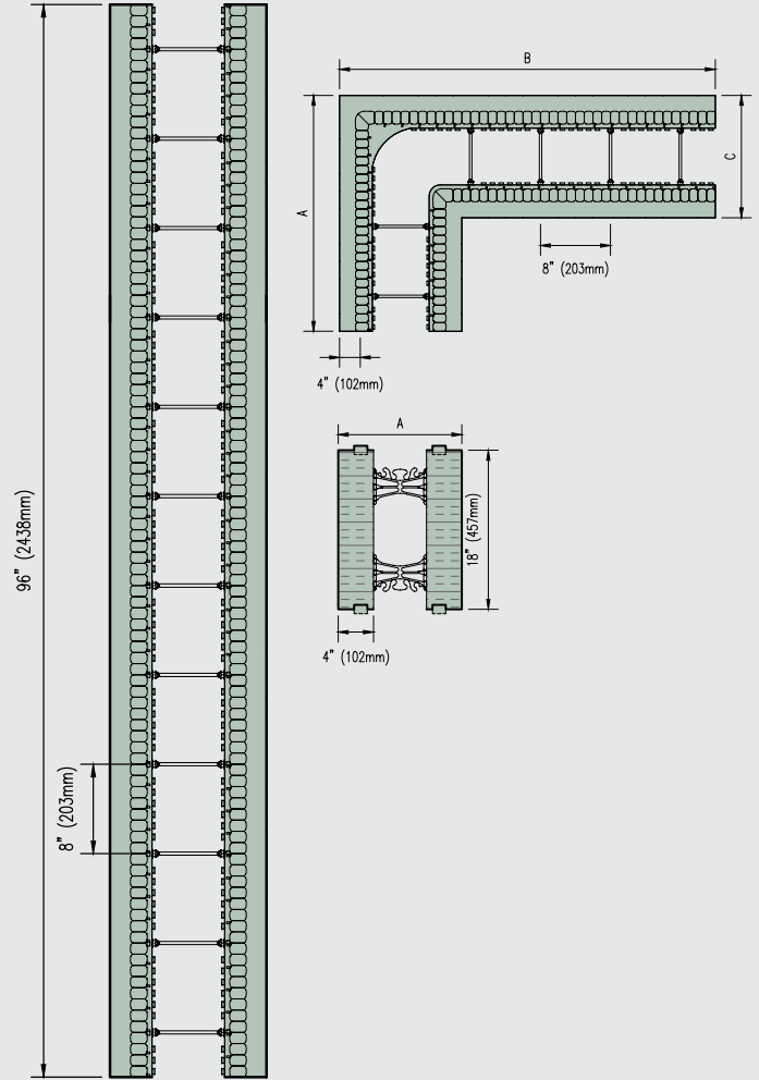
Webs are 5/8" away from the outside surface
